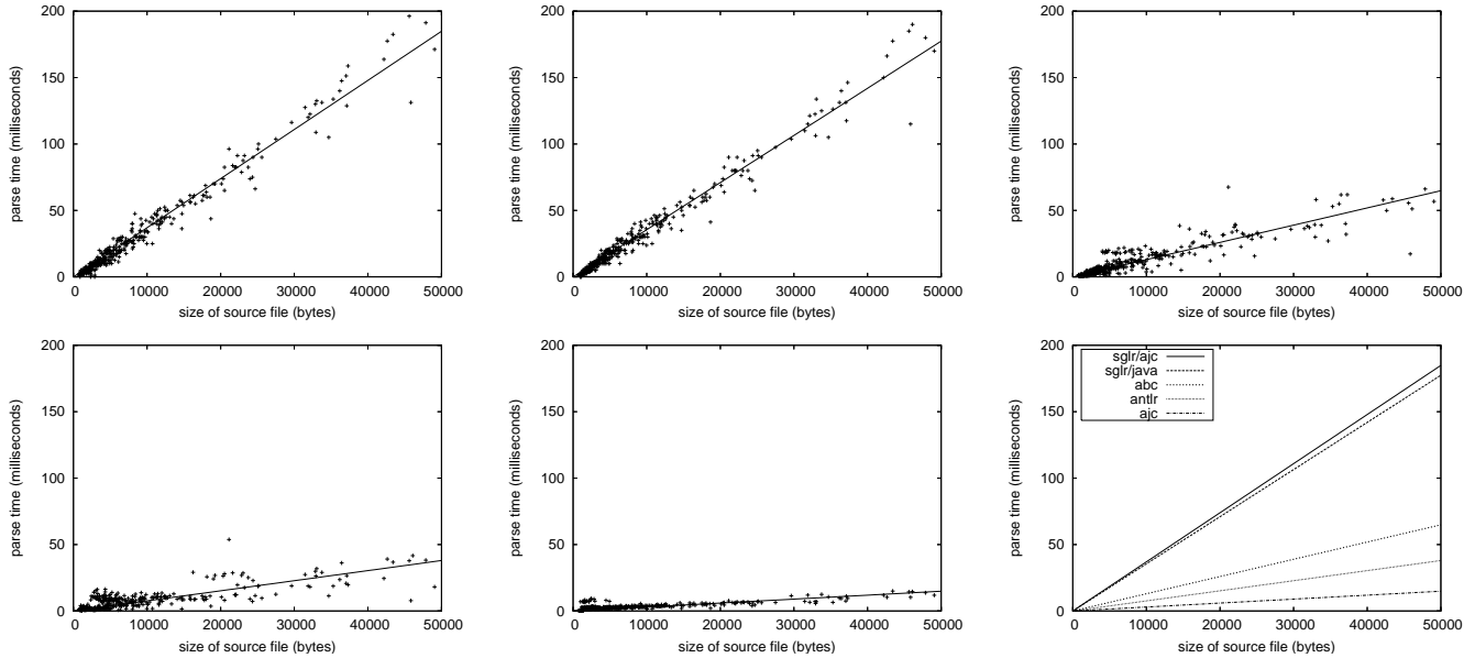
Figure 22. Benchmark of Java source files. Left to right: sgrl/ajc, sgrl/java, abc, ANTLR, ajc, and the trend lines in a single graph.
