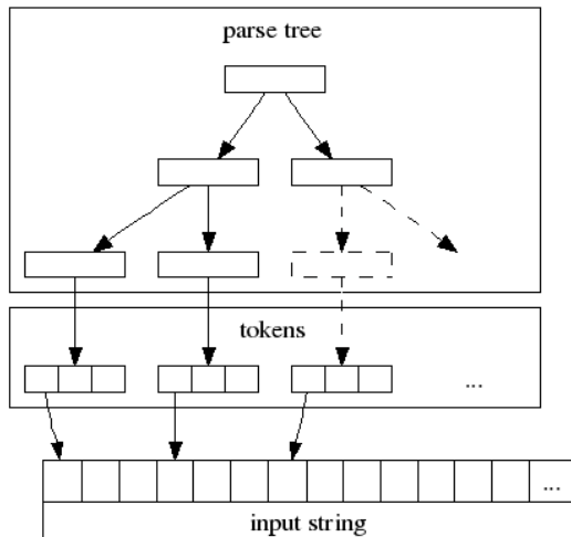
Figure 2. A scanner-based parser uses a scanner to partition the input string into tokens, which become the leaves of parse trees.
