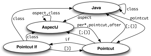
Figure 7. Lexical state transitions in the abc scanner
