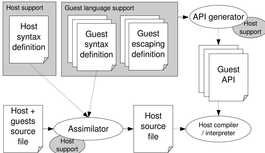
Fig. 3. Overview of the StringBorg approach
